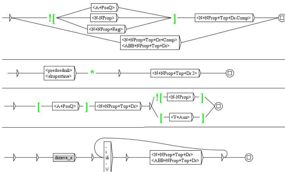
Fig. 3. Simplified sub-graphs for recognition of state names
